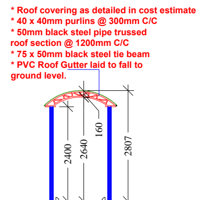
Sectional View of Walkway (B-B).
