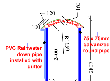
Sectional View of Walkway (A-A).
