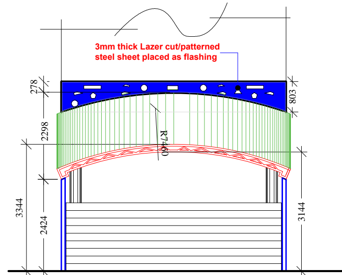
Entrance cover into the main building front view
