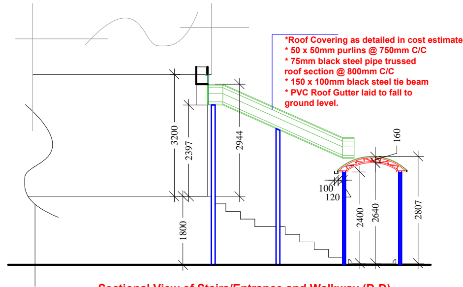
Sectional View of Stairs/Entrance and Walkway (D-D).
