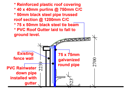
Sectional View of external entrance/visitors sitting roof covering (E-E).
