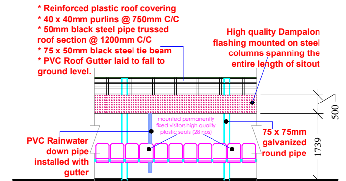
Approach View of external entrance/visitors sitting.
