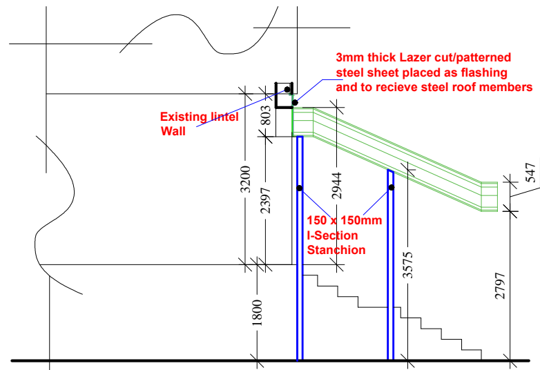
Sectional Side View of Stairs/Entrance (C-C).
