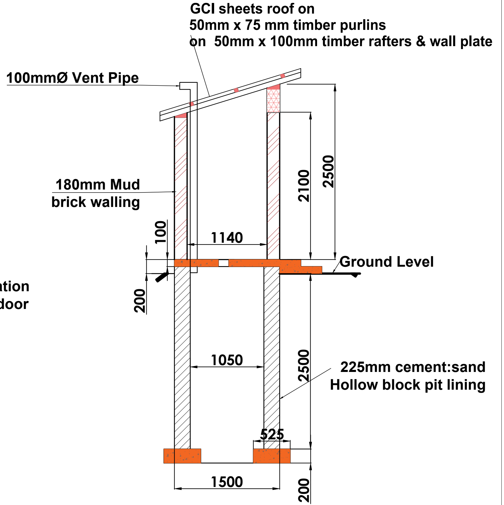
Proposed Family Pit Latrine - Pulka Shelter Project
