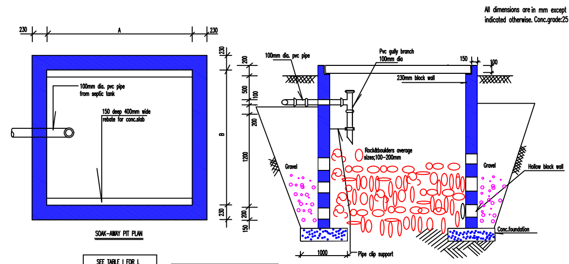
SOAK-AWAY PIT SECTION
