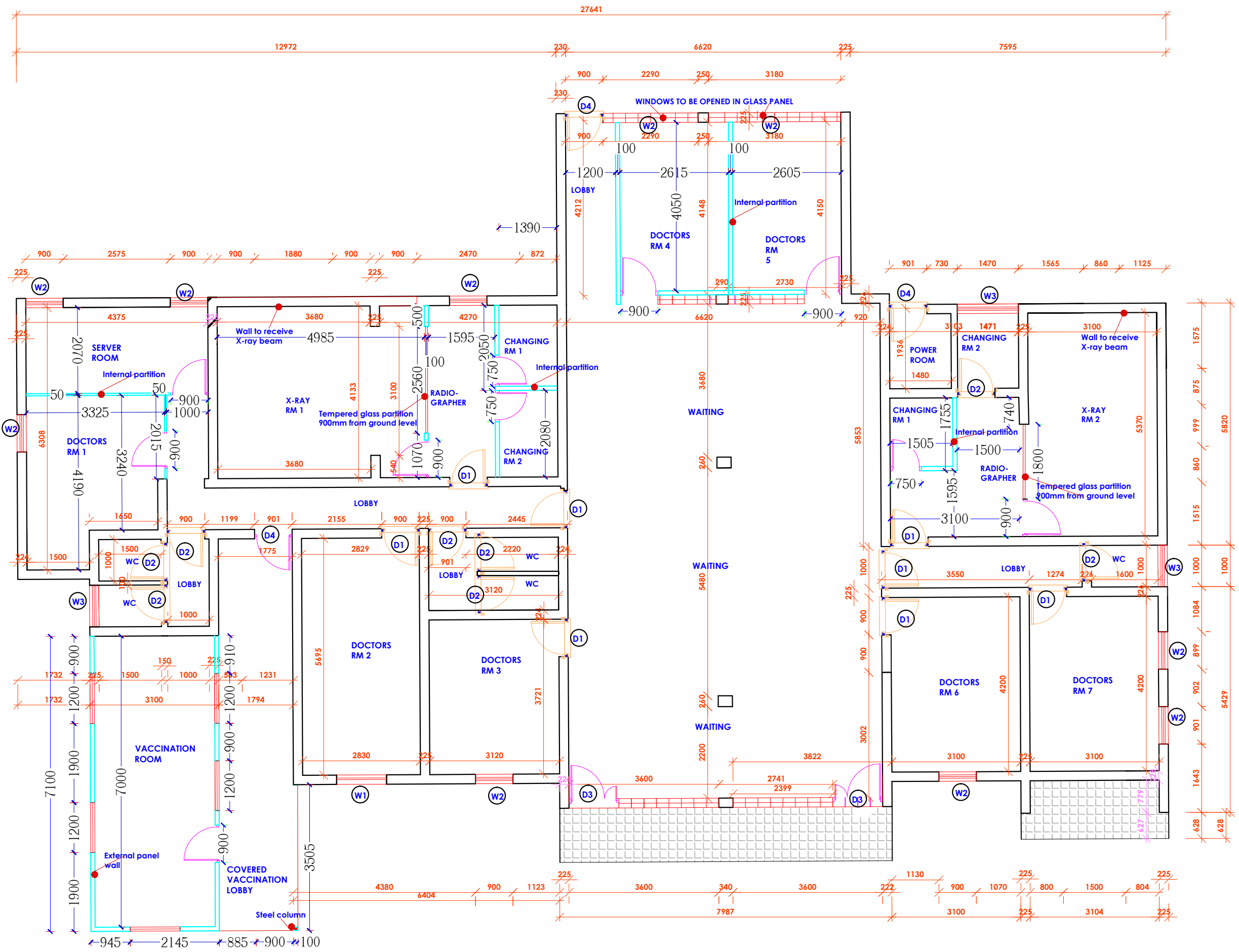
PROPOSED UPDATED BUNGALOW FLOOR PLAN
