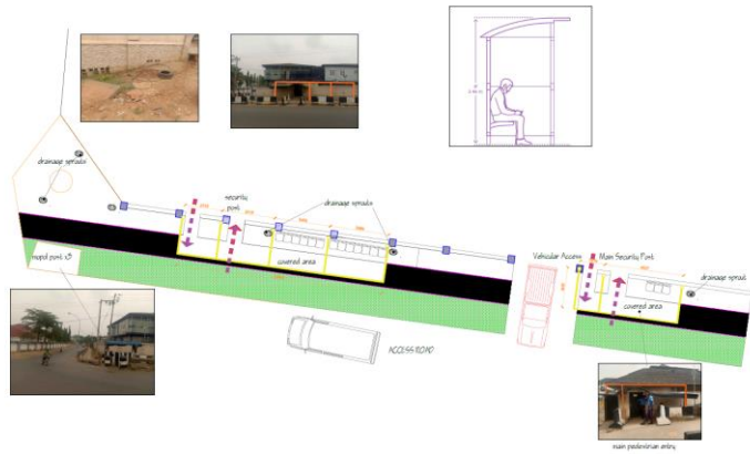
C. GRADIENT STABILIZATION AND DRAINING WITH PVC PIPES IS REQUIRED AT THESE SECTIONS
