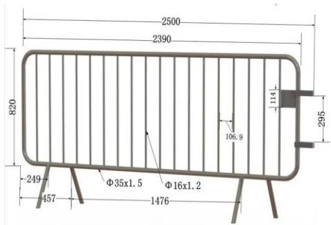
A. PEDESTRIAN CONTROL BARRIER
